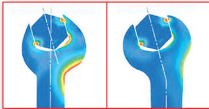
Load zones for conventional open ended spanner.
